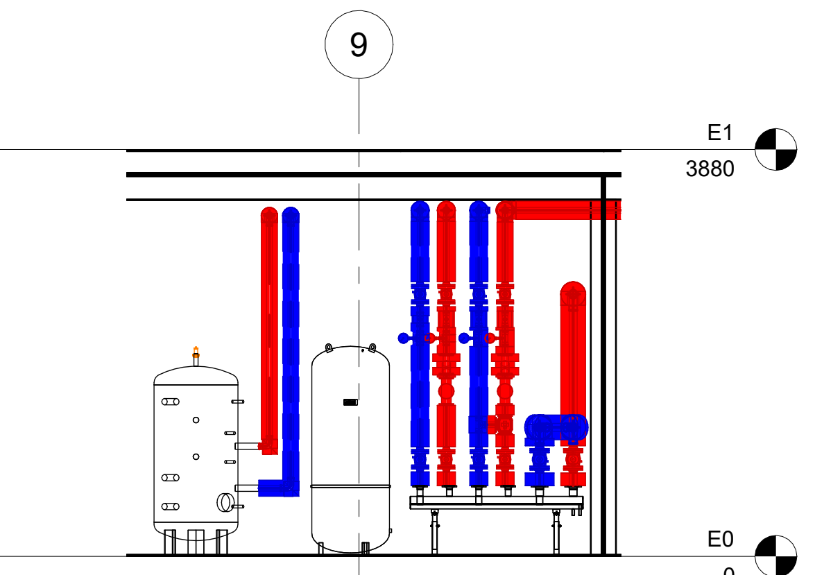
4 420_SN_Technikraum_03 1:50
