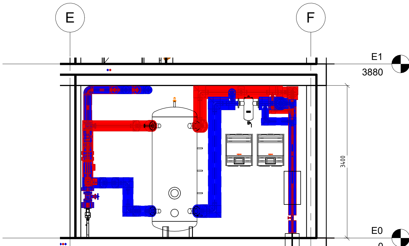
2 420_SN_Technikraum_01 1:50
