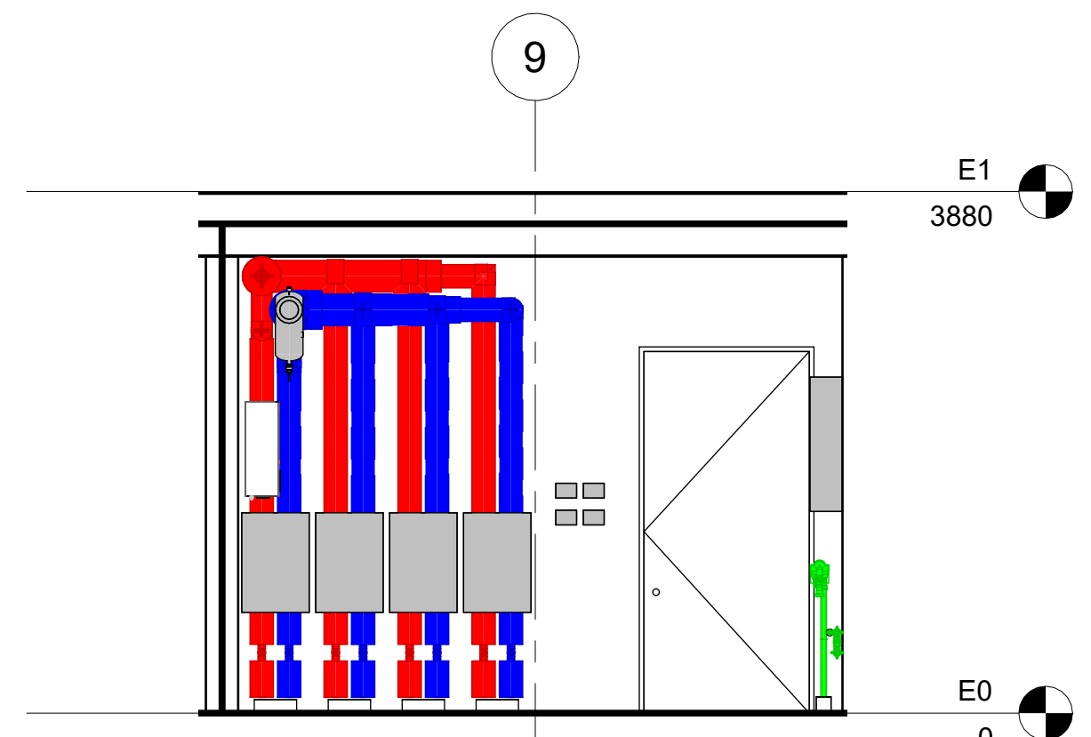
3 420_SN_Technikraum_02 1:50
